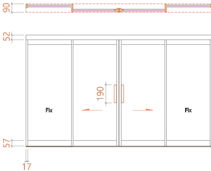
2TRACK 2SLIDING+2FIX / CORNER 2TRACK 2SLIDING+2FIX
